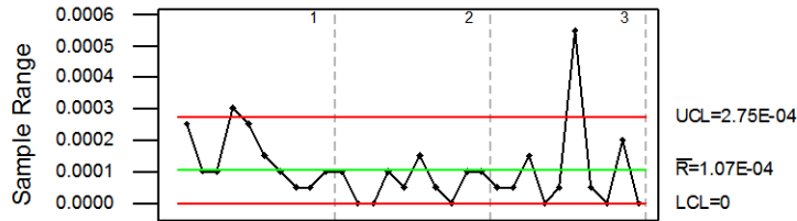
R Chart by Inspectors
