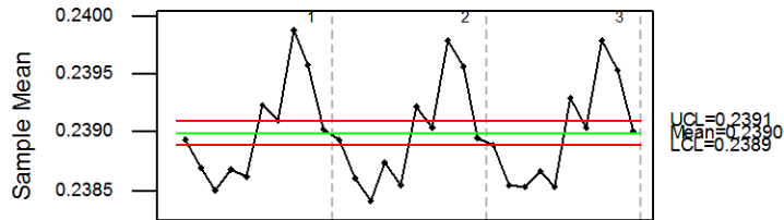
Xbar Chart by Inspectors
